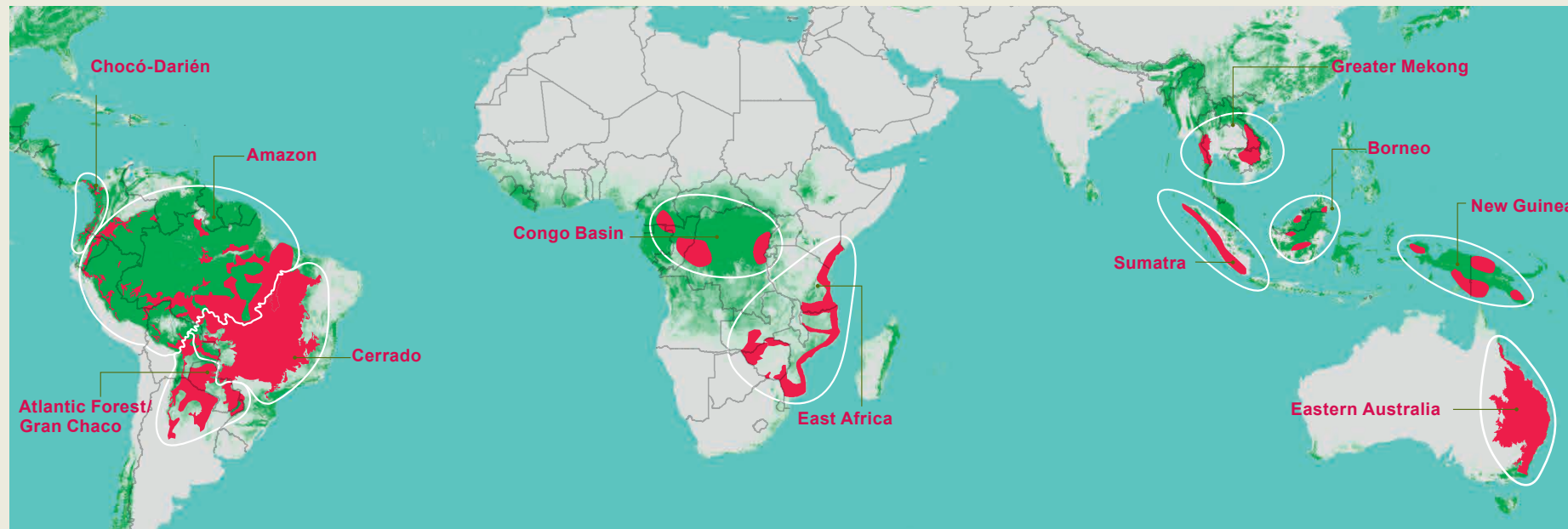
Figure 10: Hotspots of projected forest loss between 2010 and 2030 59 .
