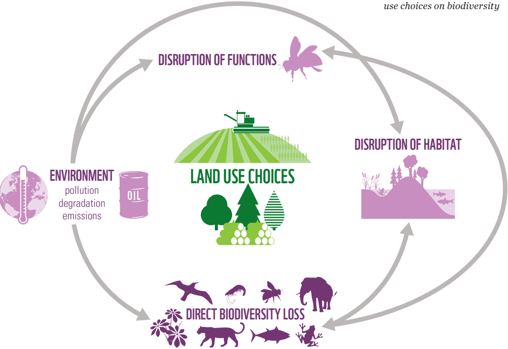
Figure 8: Direct and indirect negative impacts of land use choices on biodiversity
