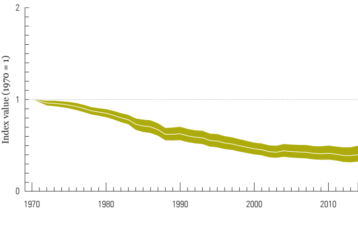
Figure 20: The Global Living Planet Index: 1970 to 2014 Average abundance of 16,704 populations representing 4,005 species monitored across the globe declined by 60%. The white line shows the index values and the shaded areas represent the statistical certainty surrounding the trend (range: -50% to -67%) 1 .
