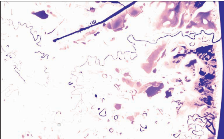
Figure 14: Rio Grande river system Shades of purple measure the length of time water has been present on the surface (darker tones equate to longer periods of time where water is present). Satellite images Landsat courtesy USGS/NASA. Global Surface Water Explorer maps courtesy JRC/Google https://global-surface-water.appspot.com
