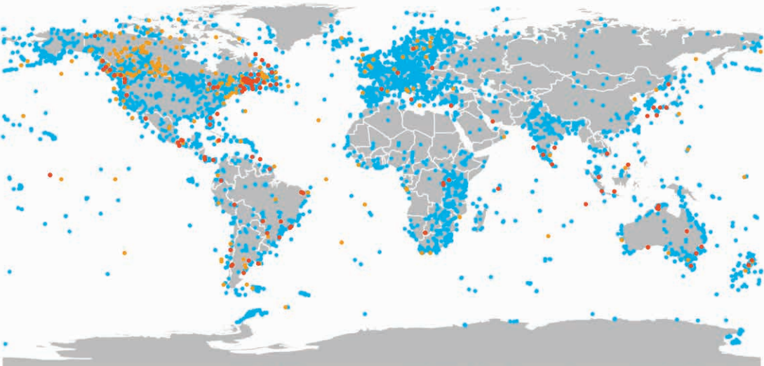
Figure 23: Locations of Living Planet Index species populations Map showing the locations of the monitored populations in the LPI. Newly added populations since the last report are highlighted in orange, or in red for species new to the LPI 1 .
