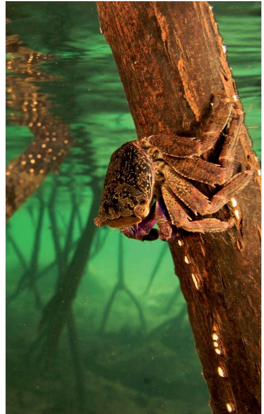
A mangrove crab on the root of a red mangrove tree ( Rhizophora mangle ), just below the water line on Kosrae Island, Federated States of Micronesia.
